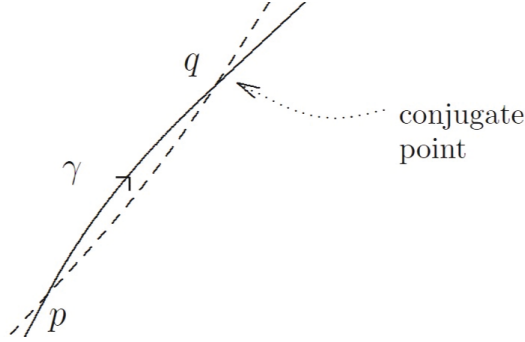
Figure 5.4: Solid line is geodesic \gamma . Geodesics near \gamma (dashed line), pass through point p and form a caustic a finite distance away. The point q is conjugate to p . Points on \gamma beyond q are timelike separated from p [119].
