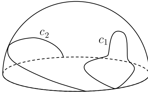
Figure 1.3: The projective space \mathcal{P}_2 with the examples of contractible ( c_1 ) and non-contractible ( c_2 ) loops.
