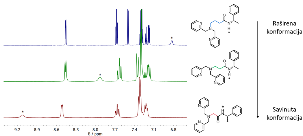
Slika 68. NMR spektri liganada \text{Db}_{1\text{A}} , \text{Db}_{2\text{A}} i \text{Db}_{3\text{A}} .
