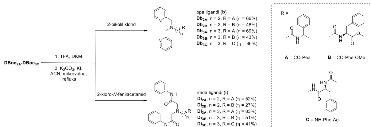
Slika 67. Shema sinteze liganada \text{Db}_{2\text{A}} - \text{Di}_{3\text{C}} .
