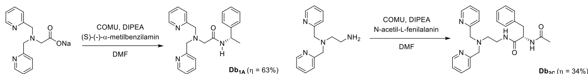
Slika 66. Shema sinteze liganada \text{Db}_{1\text{A}} i \text{Db}_{2\text{C}} .
