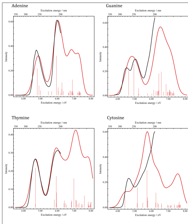
Figure 4.14: Theoretical (state-averaged, red line) and experimental (black line) UV absorption spectra of DNA nucleobases in water. Sticks indicate the mean excitation energies and oscillator strengths of the lowest 30 transitions. Figure originally published in Ref. (36).
