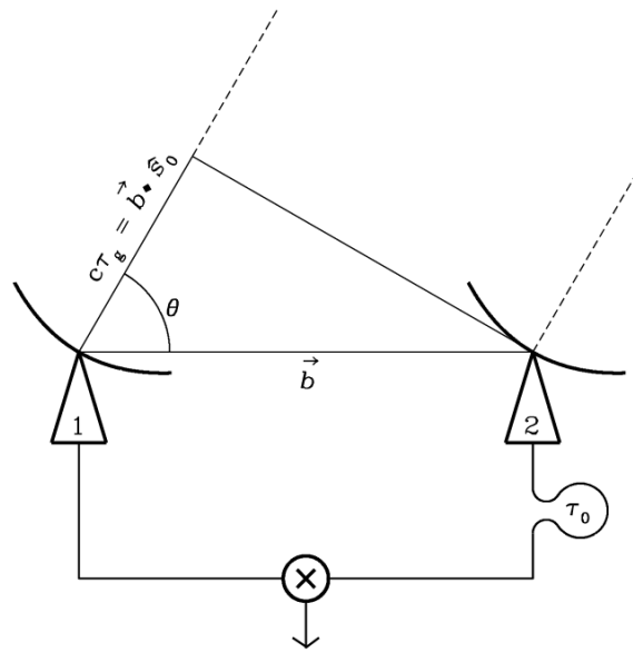
Figure 1.14: The basic element of radio interferometer is one pair of antennas. The image is taken from www.cv.nrao.edu .
