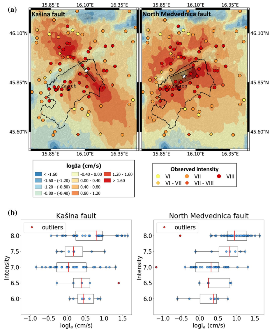
Fig. 16 a Map and b comparison of the observed intensity (MSK scale) for the 1880, M_W = 6.2 event (Herak et al. 2021) and the logarithm with base 10 of the Arias intensity calculated from the low-frequency ( f < 1 Hz) simulated waveforms for the Kašina fault and North Medvednica fault. Black line marks the boundary of the Zagreb metropolitan area
